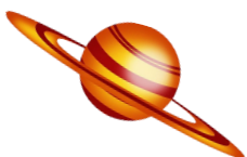
Saturn
